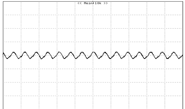
Figure 8: Output ripple & noise at 12Vin, 2.5V/3A out 50mV/div, pk-pk : 27.50mV, rms : 7.67mV(50mV/div,5uS/div)
