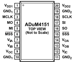
Figure 5. ADuM4151 Pin Configuration
