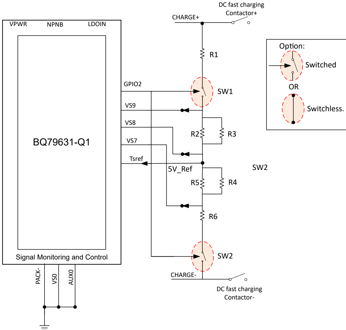
Figure 9-5. CHARGE +/- Measurement
