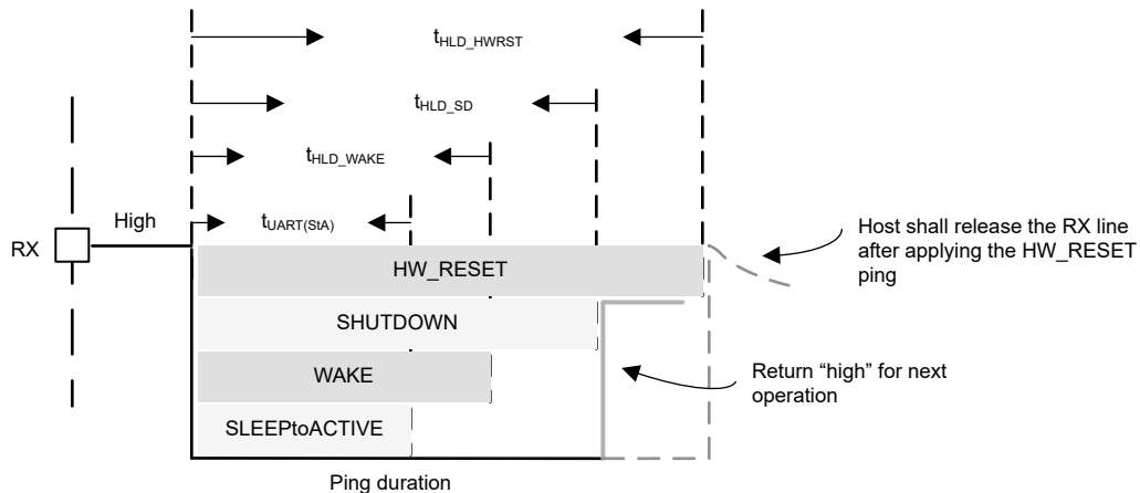
Figure 8-47. Communication Pings
