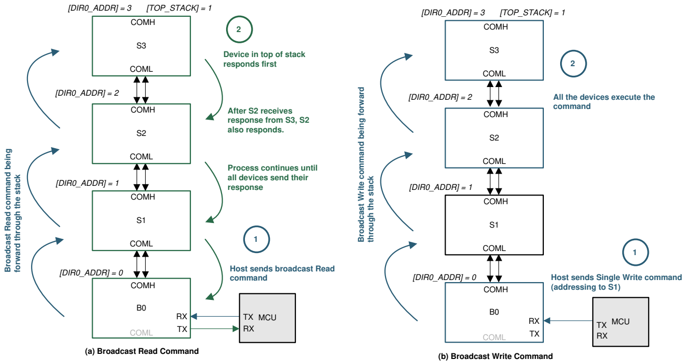
Figure 8-23. Broadcast Read/Write
