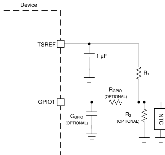
Figure 9-11. NTC Connection
