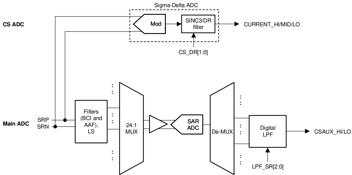
Figure 8-10. CS ADC
