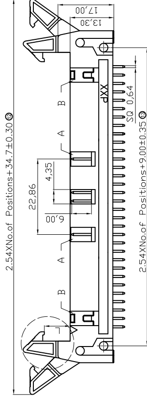
Dimension L
