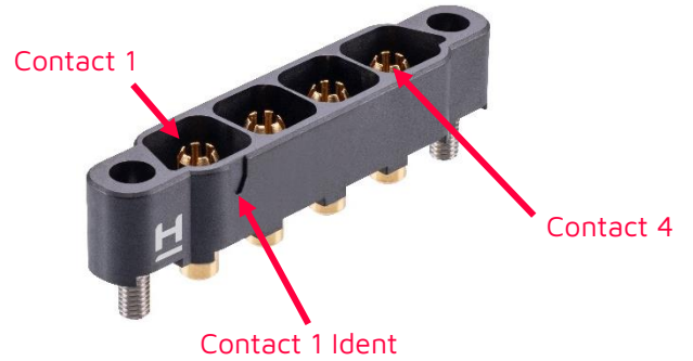
Male Connector
