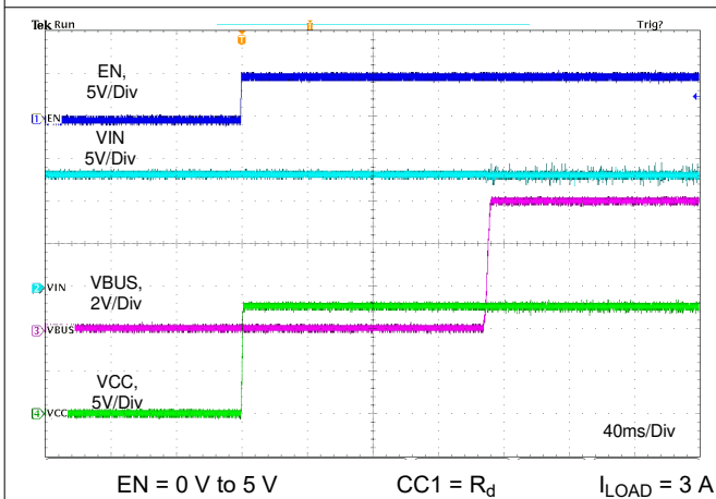
EN = 0\text{ V to }5\text{ V} CC1 = R_d I_{LOAD} = 3\text{ A} Figure 11-18. Startup Relate to EN
