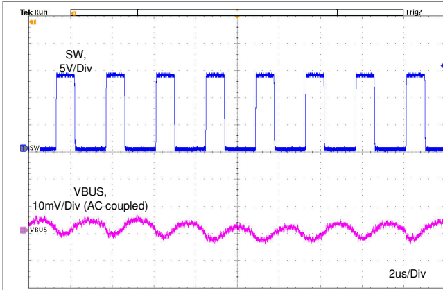
R_{IMON} = 13\text{ k}\Omega Figure 11-14. 100-mA Output Ripple
