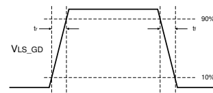
Figure 9-4. NFET Gate Drive Rise and Fall Time
