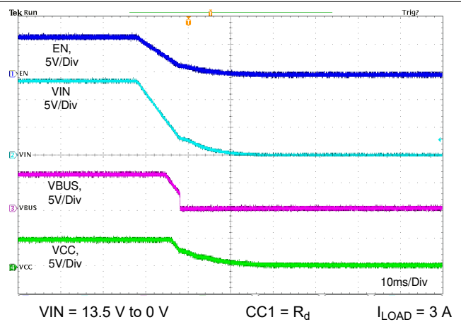
VIN = 13.5\text{ V to }0\text{ V} CC1 = R_d I_{LOAD} = 3\text{ A} Figure 11-17. Shutdown Relate to VIN
