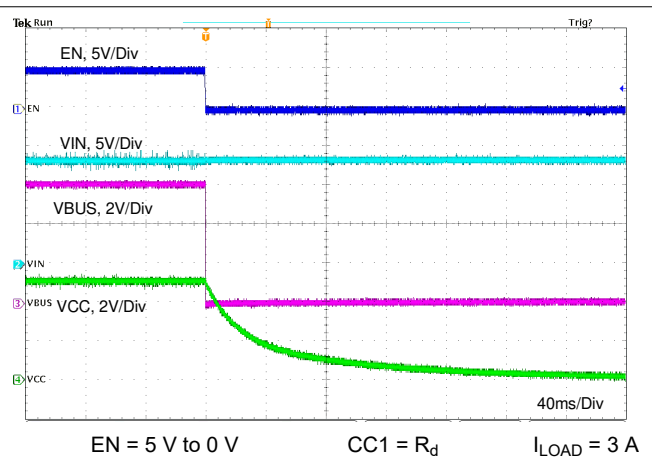
EN = 5\text{ V to }0\text{ V} CC1 = R_d I_{LOAD} = 3\text{ A} Figure 11-19. Shutdown Relate to EN
