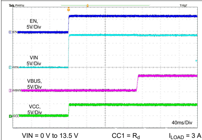
VIN = 0\text{ V to }13.5\text{ V} CC1 = R_d I_{LOAD} = 3\text{ A} Figure 11-16. Startup Relate to VIN
