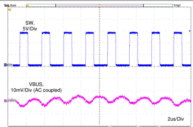
R_{IMON} = 13\text{ k}\Omega Figure 11-15. No Load Output Ripple
