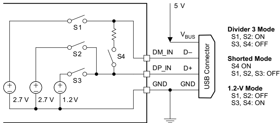
Figure 10-35. DCP Auto Mode
