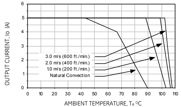
Figure 58. Derating Output Current versus Local Ambient Temperature and Airflow.
