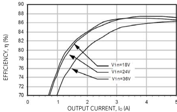
Figure 55. Converter Efficiency versus Output Current.
