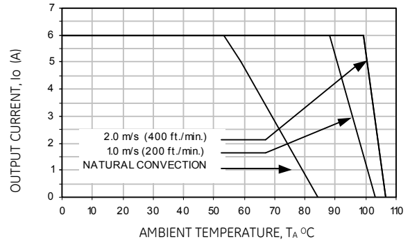
Figure 16. Derating Output Current versus Local Ambient Temperature and Airflow.
