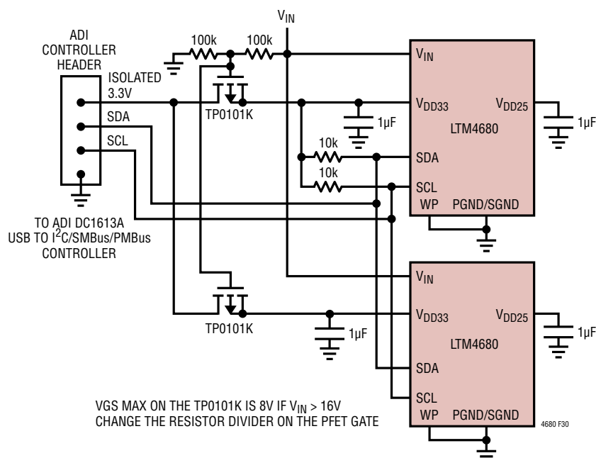
Figure 30. Controller Connection
