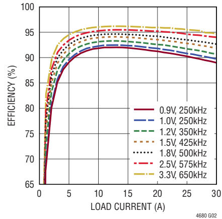
Single Channel Efficiency, 8V IN , V IN = SV IN = 8V, EXT CC = 5V, CCM Mode
