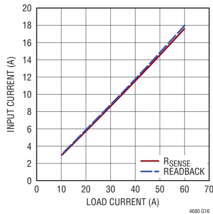
Supply Current vs Load Current Comparison, R_{\text{SENSE}} = 3\text{m}\Omega , 12\text{V} to 3.3\text{V}_{\text{OUT}} , 650\text{kHz}
