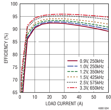
Dual Channel Single Output Efficiency, 12V IN , V IN = SV IN = 12V, EXT CC = 5V, V OUT0 and V OUT1 Paralleled, CCM Mode
