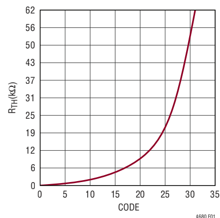
Figure 1. Programmable R_{COMP}
