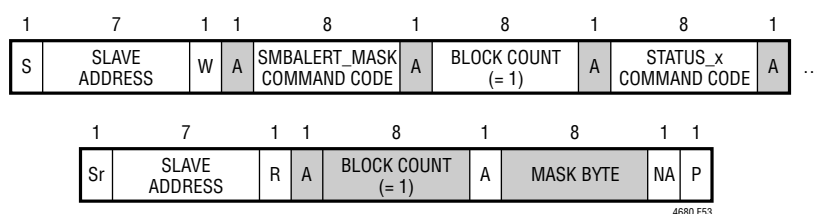
Figure 53. Example of Reading SMBALERT_MASK
