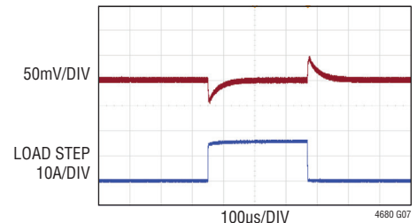
FIGURE 46 CIRCUIT, 12V TO 1.8V, FREQ = 500kHz C_{OUT} = 470\mu\text{F} \times 2 POSCAP, 100\mu\text{F} \times 4 CERAMIC R_{COMP} = 17\text{k} , EA-GM = 3.69ms, COMP_{Pa} = 3.3\text{nF} , COMP_{Pb} = 68\text{pF} I_{LIM} LOW, V_{OUT} RANGE LOW
