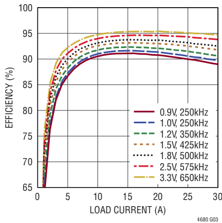
Single Channel Efficiency, 12V IN , V IN = SV IN = 12V, EXT CC = 5V, CCM Mode
