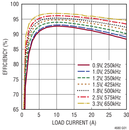
Single Channel Efficiency, 5V IN , V IN = SV IN = EXT CC = 5V, CCM Mode
