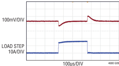
FIGURE 46 CIRCUIT, 12V TO 3.3V, FREQ = 650kHz C_{OUT} = 470\mu\text{F} \times 2 POSCAP, 100\mu\text{F} \times 4 CERAMIC R_{COMP} = 20\text{k} , EA-GM = 3.02ms, COMP_{Pa} = 3.3\text{nF} , COMP_{Pb} = 68\text{pF} I_{LIM} LOW, V_{OUT} RANGE HIGH
