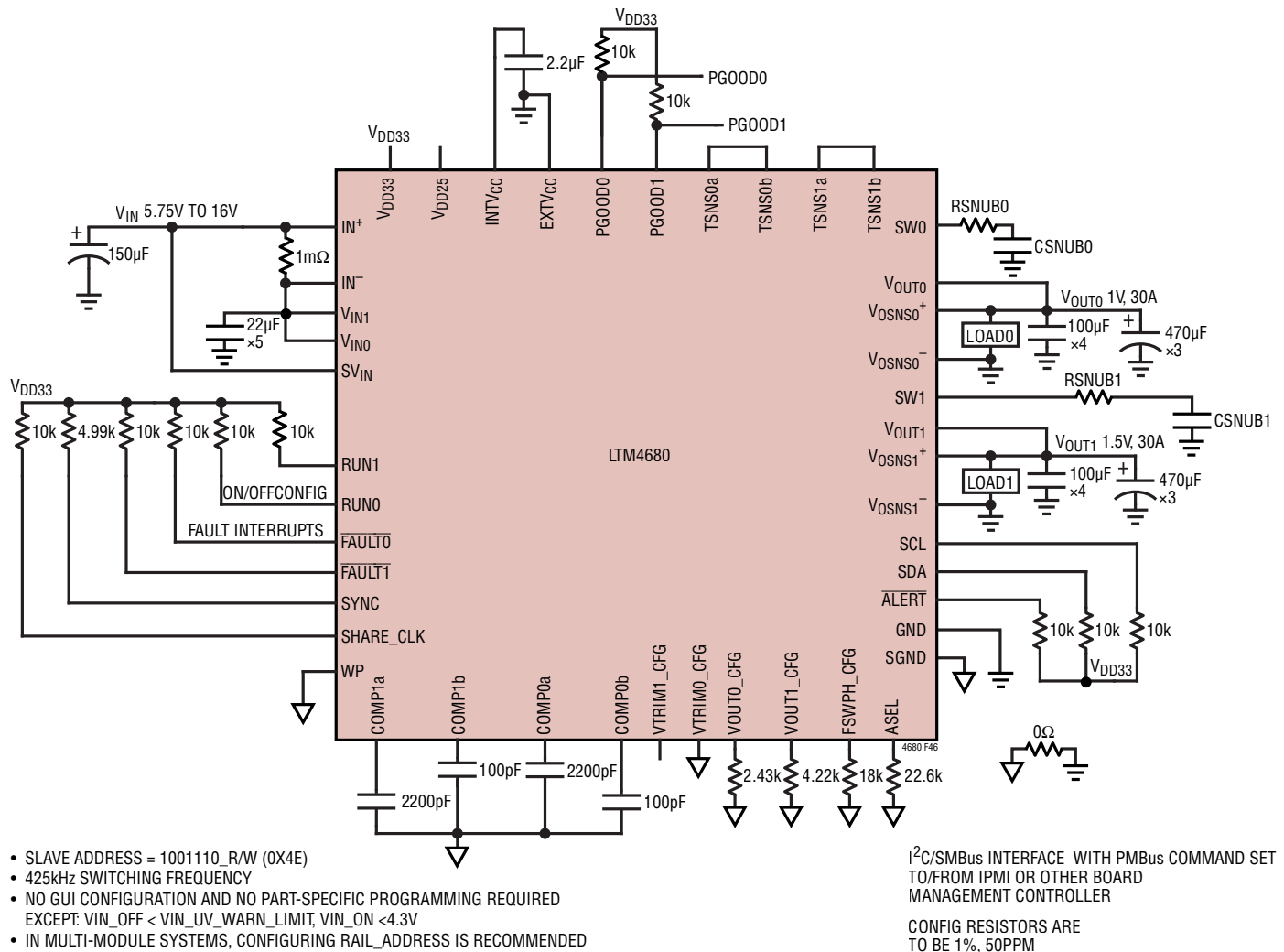
Figure 46. 1.0V and 1.5V Outputs at 30A With Providing I 2 C/SMBus/PMBus Serial Interface
