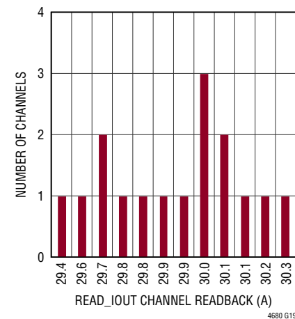
READ_IOUT of 16 LTM4680 Channels
