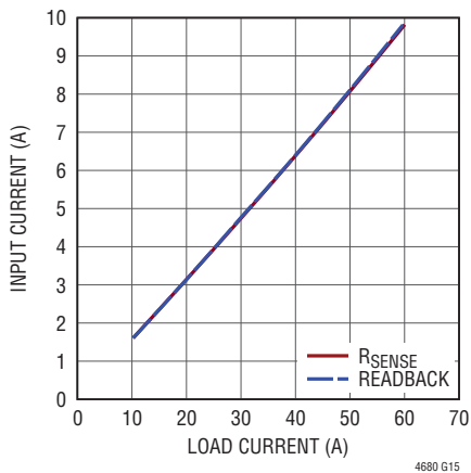
Supply Current vs Load Current Comparison, R_{\text{SENSE}} = 3\text{m}\Omega , 12\text{V} to 1.8\text{V}_{\text{OUT}} , 500\text{kHz}
