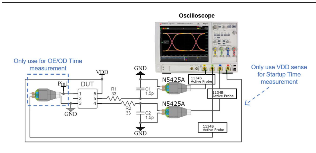
Figure 16. Test setup to measure Low-Power HCSL Waveform Characteristics, Current Consumption, Output Enable/Disable Time, and Startup Time
