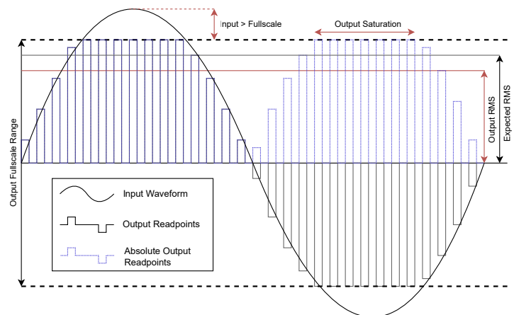
Figure 20: Output Saturation
