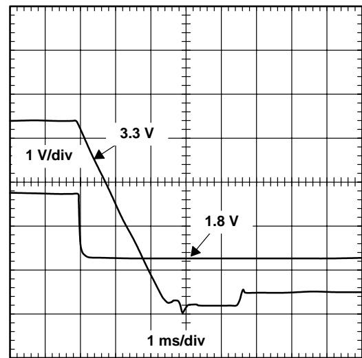
POWER-DOWN SEQUENCING
