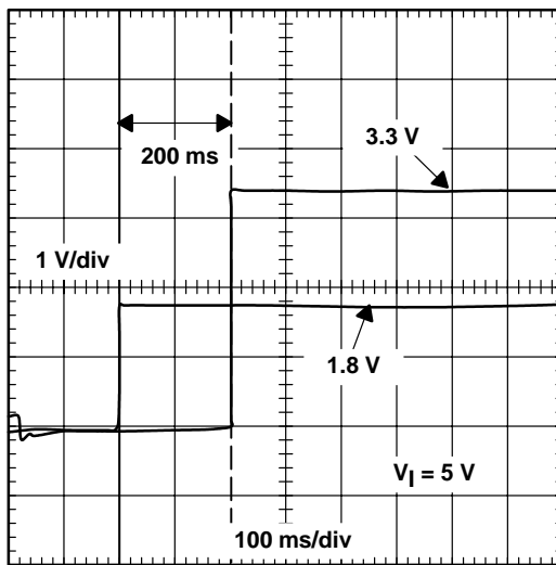
POWER-UP SEQUENCING
