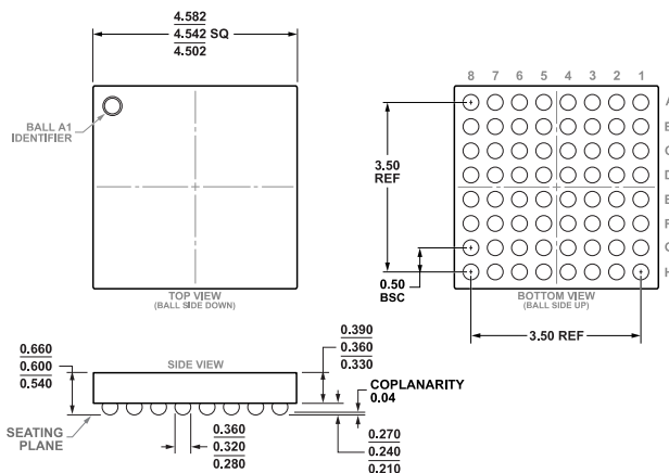
Figure 62. 64-Ball Wafer Level Chip Scale Package [WLCSF] (CB-64-5) Dimensions shown in millimeters
