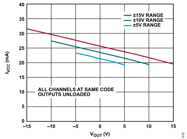
Figure 13. I_{ICC} vs. V_{OUT}
