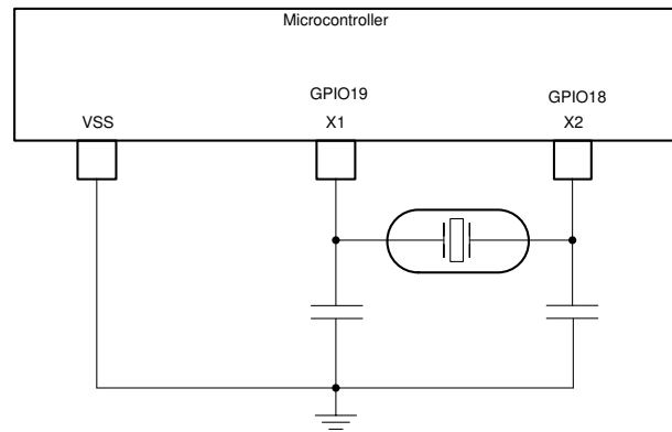
Figure 6-16. External Crystal
