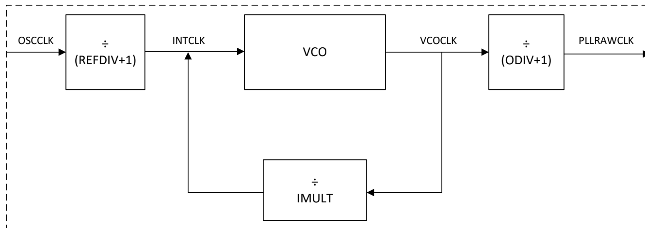
Figure 6-14. System PLL
