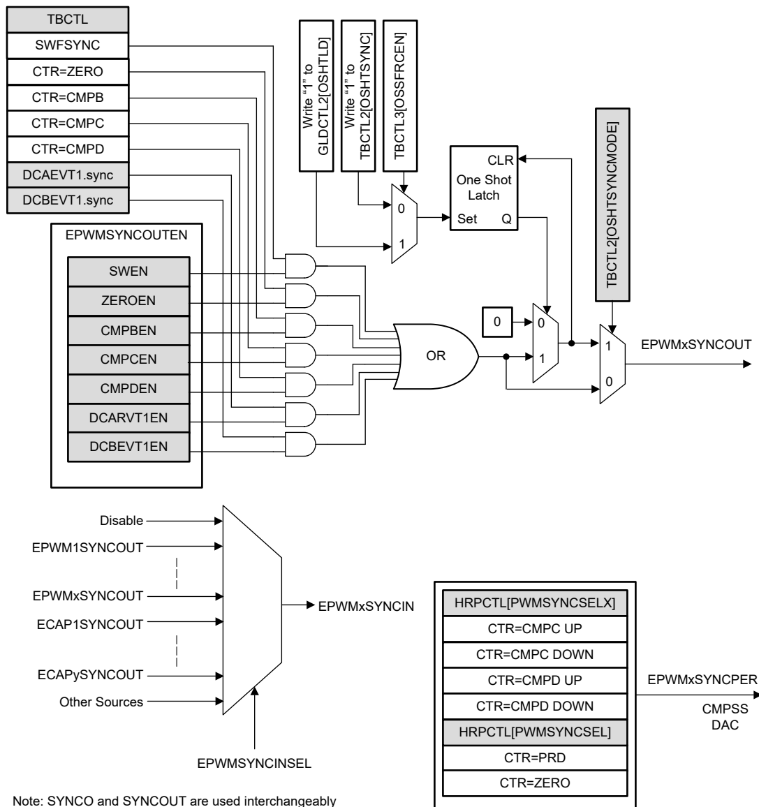
Figure 6-52. Synchronization Chain Architecture
