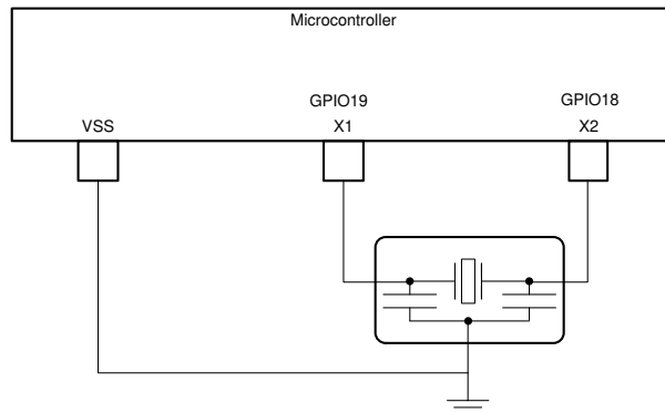
Figure 6-17. External Resonator
