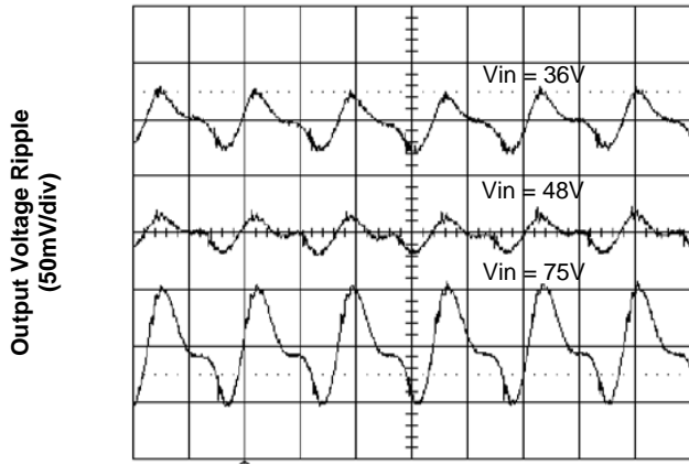
Figure 3. Output Ripple Voltage at Full Load
