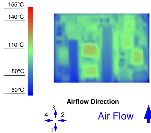
Figure 8. Thermal Image for Airflow Direction 3 (20.5A output, 55°C ambient, 0 LFM, typical Vin, open frame, unit soldered onto a fixture board)
