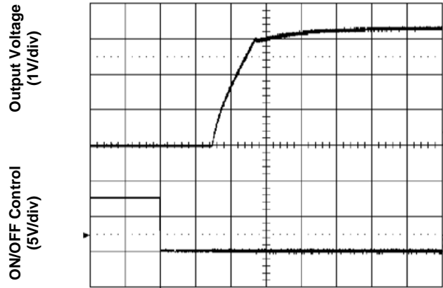
Figure 4. Start-Up from Enable Control (typical Vin, full load)
