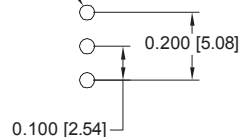
CONTACT HOLE PATTERN
