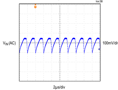
MAXM15063 INPUT VOLTAGE RIPPLE V_{IN} = 48V , FIXED V_{OUT} = 5V , FULL LOAD, PWM MODE
