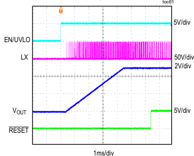
MAXM15063 STARTUP THROUGH ENABLE V_{IN} = 48V , FIXED V_{OUT} = 5V , FULL LOAD, PWM MODE
