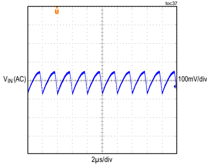
MAXM15062 INPUT VOLTAGE RIPPLE V_{IN} = 24V , FIXED V_{OUT} = 3.3V , FULL LOAD, PWM MODE
