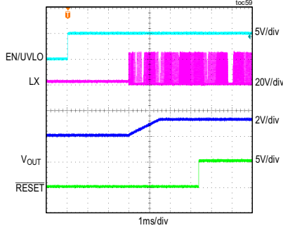
MAXM15062 STARTUP THROUGH ENABLE (2V PREBIAS) V_{IN} = 24V , FIXED V_{OUT} = 3.3V , NO LOAD, PWM MODE
