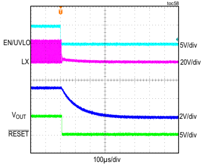
MAXM15062 SHUTDOWN THROUGH ENABLE V_{IN} = 24V , FIXED V_{OUT} = 3.3V , FULL LOAD, PWM MODE
