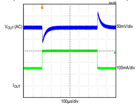
MAXM15063 LOAD TRANSIENT RESPONSE V_{IN} = 48V , FIXED V_{OUT} = 5V , PWM MODE (LOAD CURRENT STEPPED FROM 150mA TO 300mA)
