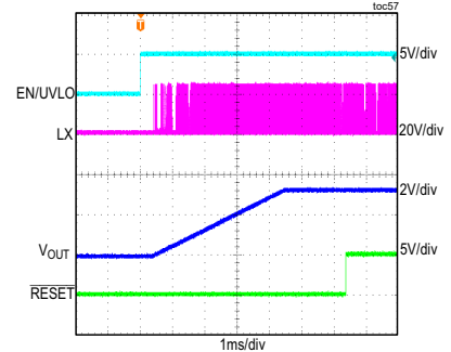
MAXM15062 STARTUP THROUGH ENABLE V_{IN} = 24V , FIXED V_{OUT} = 3.3V , FULL LOAD, PWM MODE
