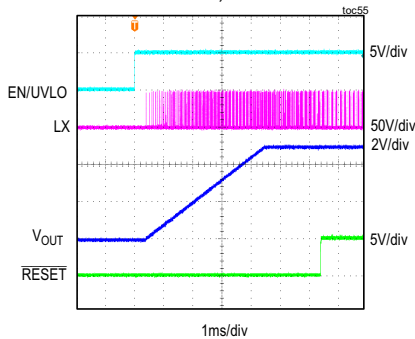
MAXM15064 STARTUP THROUGH ENABLE V_{IN} = 48V , ADJUSTABLE V_{OUT} = 5V , FULL LOAD, PWM MODE
