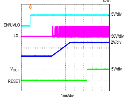
MAXM15063 STARTUP THROUGH ENABLE (2.5V PREBIAS) V_{IN} = 48V , FIXED V_{OUT} = 5V , NO LOAD, PWM MODE
