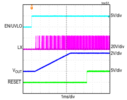
MAXM15064 STARTUP THROUGH ENABLE V_{IN} = 24V , ADJUSTABLE V_{OUT} = 3.3V , FULL LOAD, PWM MODE
