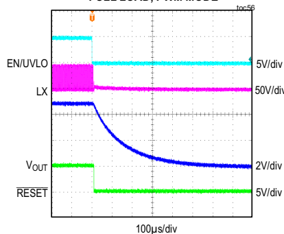
MAXM15064 SHUTDOWN THROUGH ENABLE V_{IN} = 48V , ADJUSTABLE V_{OUT} = 5V , FULL LOAD, PWM MODE
