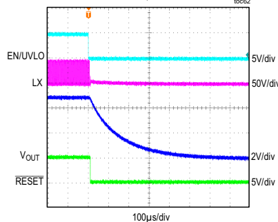
MAXM15063 SHUTDOWN THROUGH ENABLE V_{IN} = 48V , FIXED V_{OUT} = 5V , FULL LOAD, PWM MODE
