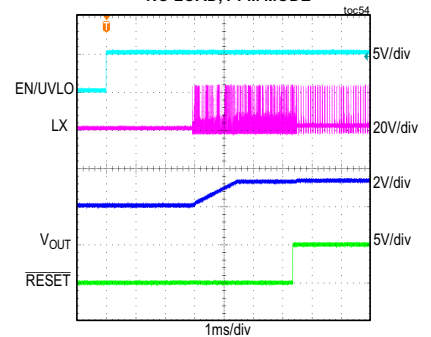
MAXM15064 STARTUP THROUGH ENABLE (2V PREBIAS) V_{IN} = 24V , ADJUSTABLE V_{OUT} = 3.3V , NO LOAD, PFM MODE
