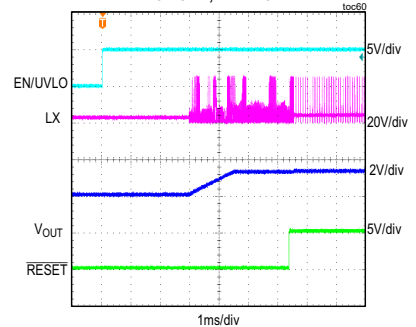
MAXM15062 STARTUP THROUGH ENABLE (2V PREBIAS) V_{IN} = 24V , FIXED V_{OUT} = 3.3V , NO LOAD, PFM MODE
