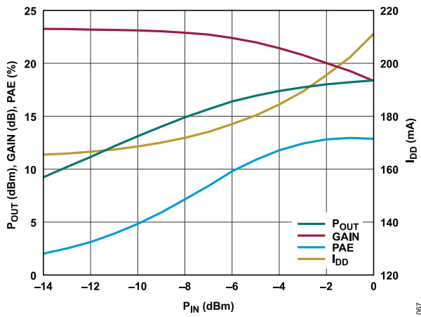
Figure 67. P_{OUT} , Gain, PAE, and I_{DQ} vs. P_{IN} , 28 GHz, V_{DD} = 2.5 V, I_{DQ} = 160 mA
