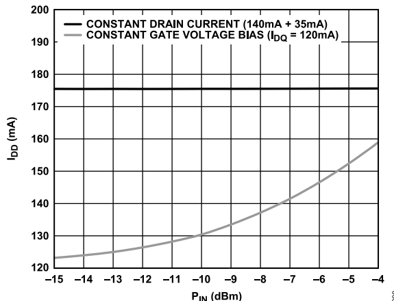
Figure 90. I_{DD} vs. P_{IN} , V_{DD} = 3 V, Frequency = 36 GHz, Constant Drain Current Bias (140 mA + 35 mA) and Constant Gate Voltage Bias ( I_{DQ} = 120 mA)
