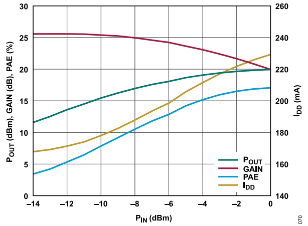
Figure 70. P_{OUT} , Gain, PAE, and I_{DQ} vs. P_{IN} , 48 GHz, V_{DD} = 2.5 V, I_{DQ} = 160 mA
