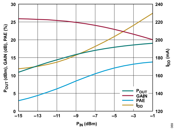
Figure 69. P_{OUT} , Gain, PAE, and I_{DQ} vs. P_{IN} , 36 GHz, V_{DD} = 2.5 V, I_{DQ} = 160 mA
