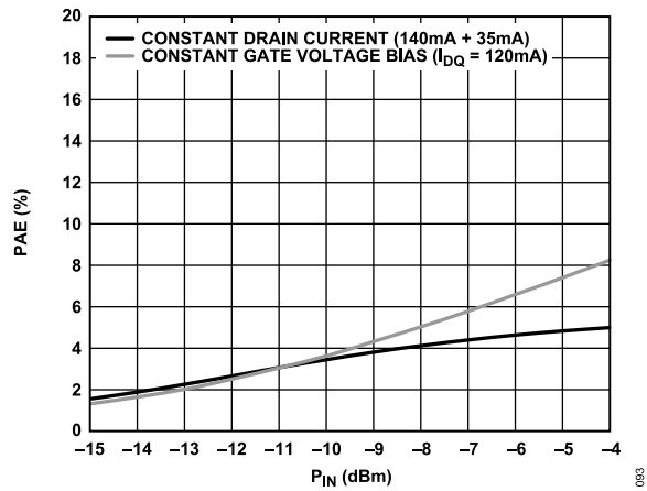
Figure 93. PAE vs. P_{IN} , V_{DD} = 3\text{ V} , Frequency = 36 GHz, Constant Drain Current Bias (140 mA + 35 mA) and Constant Gate Voltage Bias ( I_{DQ} = 120\text{ mA} )
