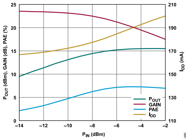
Figure 66. P_{OUT} , Gain, PAE, and I_{DQ} vs. P_{IN} , 20 GHz, V_{DD} = 2.5 V, I_{DQ} = 160 mA
