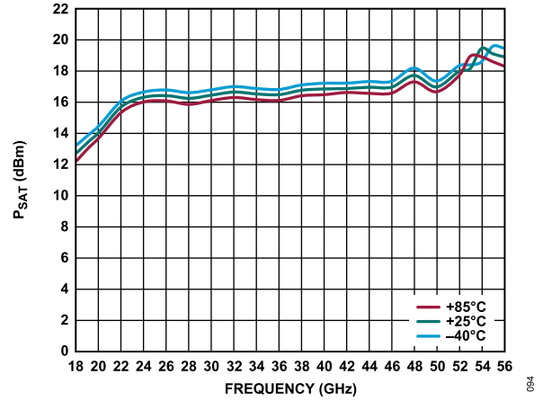
Figure 94. P_{SAT} vs. Frequency for Various Temperatures, Data Measured with I_{DQ} = 140\text{ mA}
