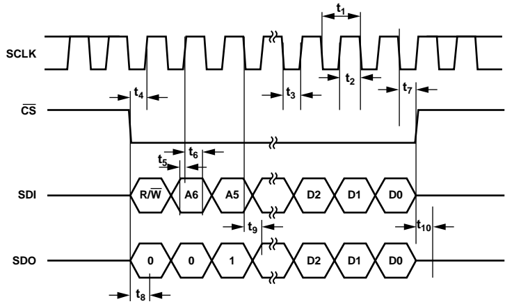
Figure 2. Address Mode Timing Diagram
