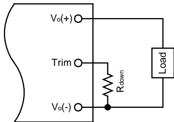
Figure 15. Circuit to Decrease Output Voltage
