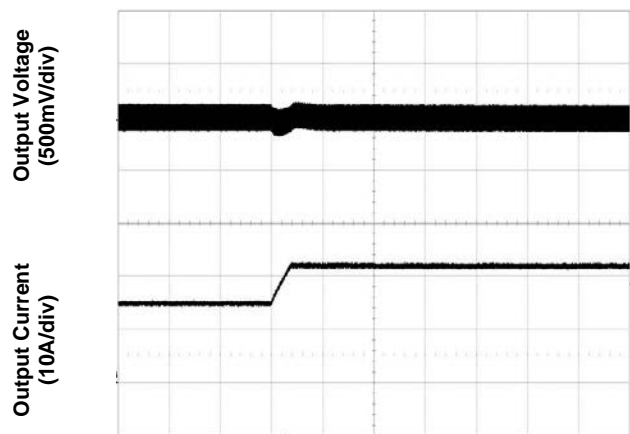
Figure 6. Transient Load Response (typical Vin, load current steps from 50% to 75% at a slew rate 0.1A/µs, 1,000µF external output capacitance)
