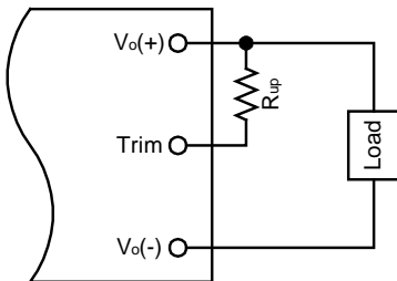
Figure 16. Circuit to Increase Output Voltage
