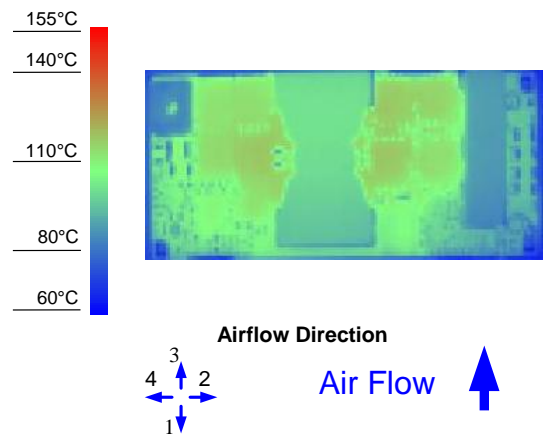
Figure 10. Thermal Image for Airflow Direction 3 (20A output, 55°C ambient, 200 LFM, typical Vin, open frame unit, solder interface)
