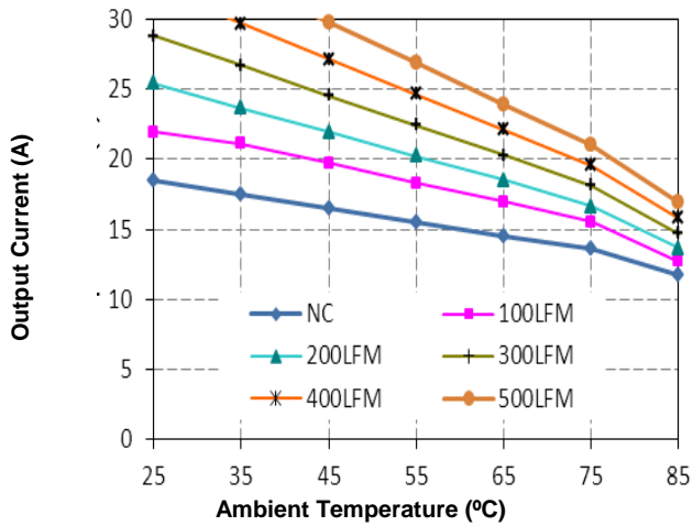
Figure 9. Current Derating Curve for Airflow Direction 3 (Ref. Fig. 10 for Airflow Direction; typical Vin, open frame unit, solder interface)
