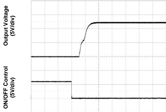
Figure 4. Start-Up from Enable Control
