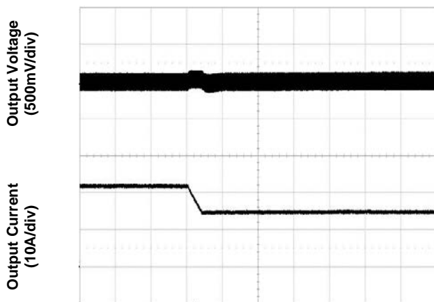
Figure 5. Transient Load Response (typical Vin, load current steps from 75% to 50% at a slew rate 0.1A/µs, 1,000µF external output capacitance)
