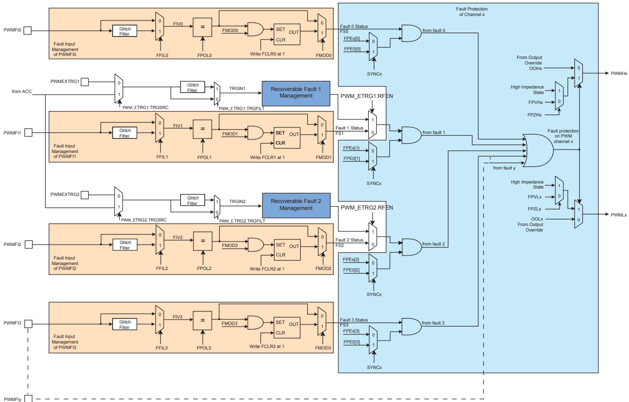
Figure 42-16. Fault Protection
