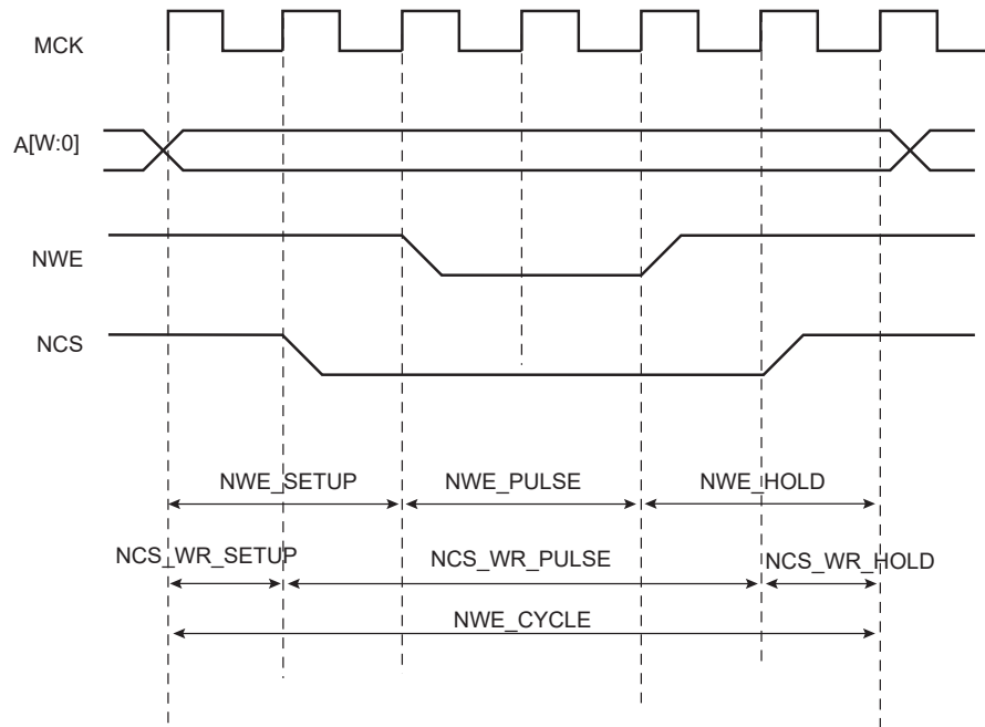
Figure 31-5. Write Cycle
