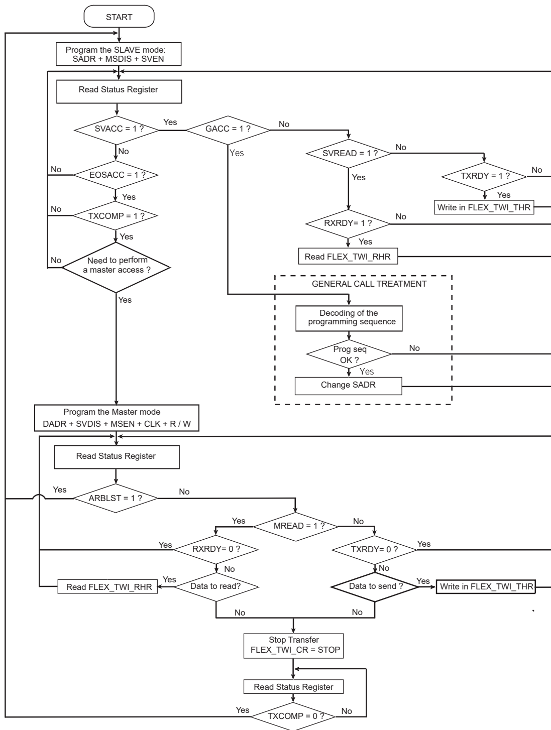
Figure 39-119. Multi-Master Mode
