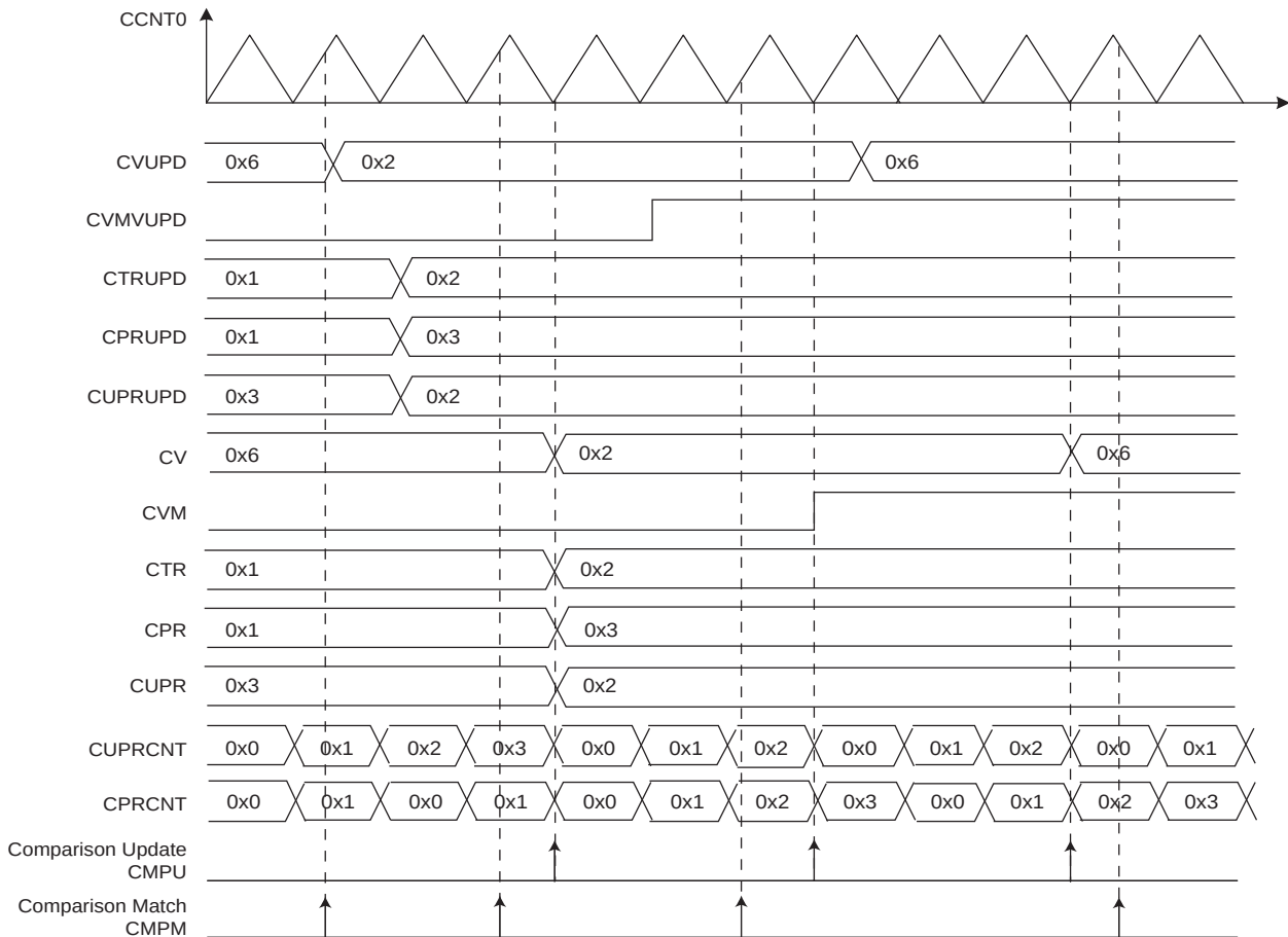
Figure 42-24. Comparison Waveform
