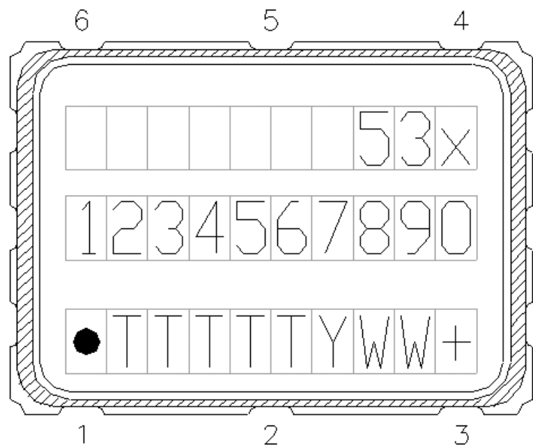
Figure 3. Mark Specification
