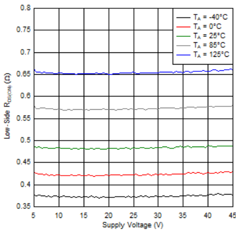
Figure 6-5. Low-Side R_{DS(ON)} over VM
