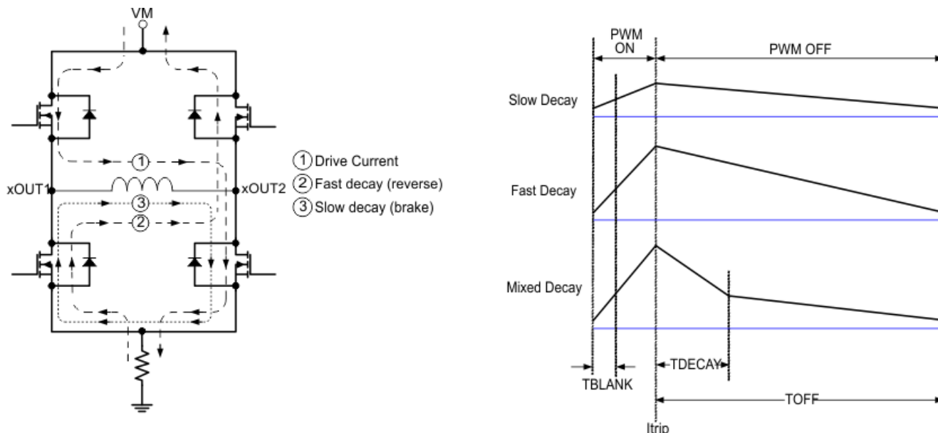
Figure 7-5. Decay Modes
