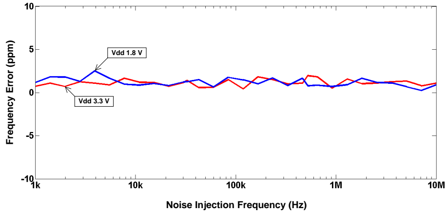
Figure 13. Power Supply Noise Rejection ( \pm 150 mV Noise)
