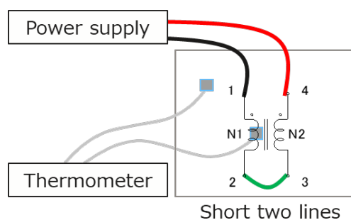
Figure 2 - Schematics
