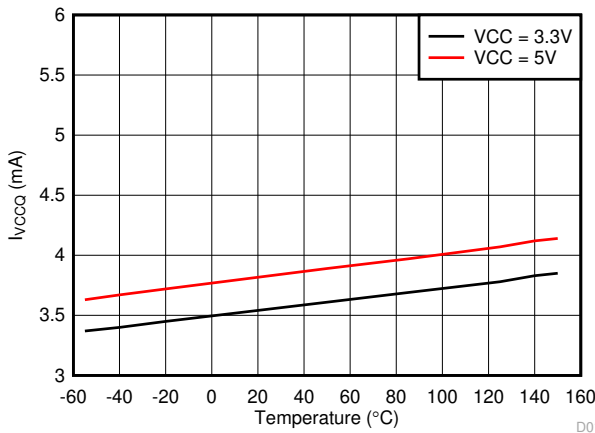
Figure 6-6. I VCCQ Supply Current vs. Temperature IN+ = High IN- = Low
