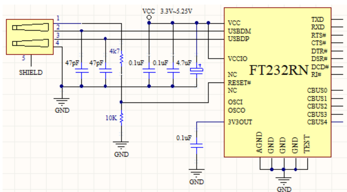
Figure 6.2 Self-Powered Configuration
