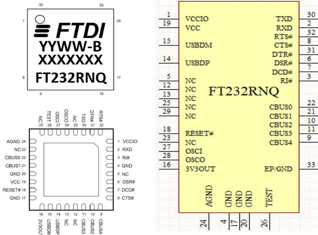
Figure 3.2 QFN-32 Package Pin Out and schematic symbol
