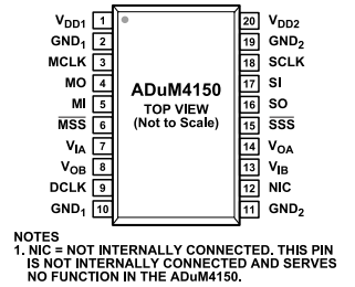
Figure 3. Pin Configuration
