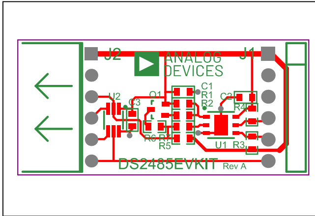
DS9121BQ Socket Board Layout Diagram—Top
