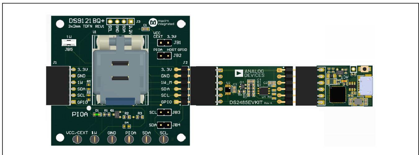
Figure 2. Board Connectivity
