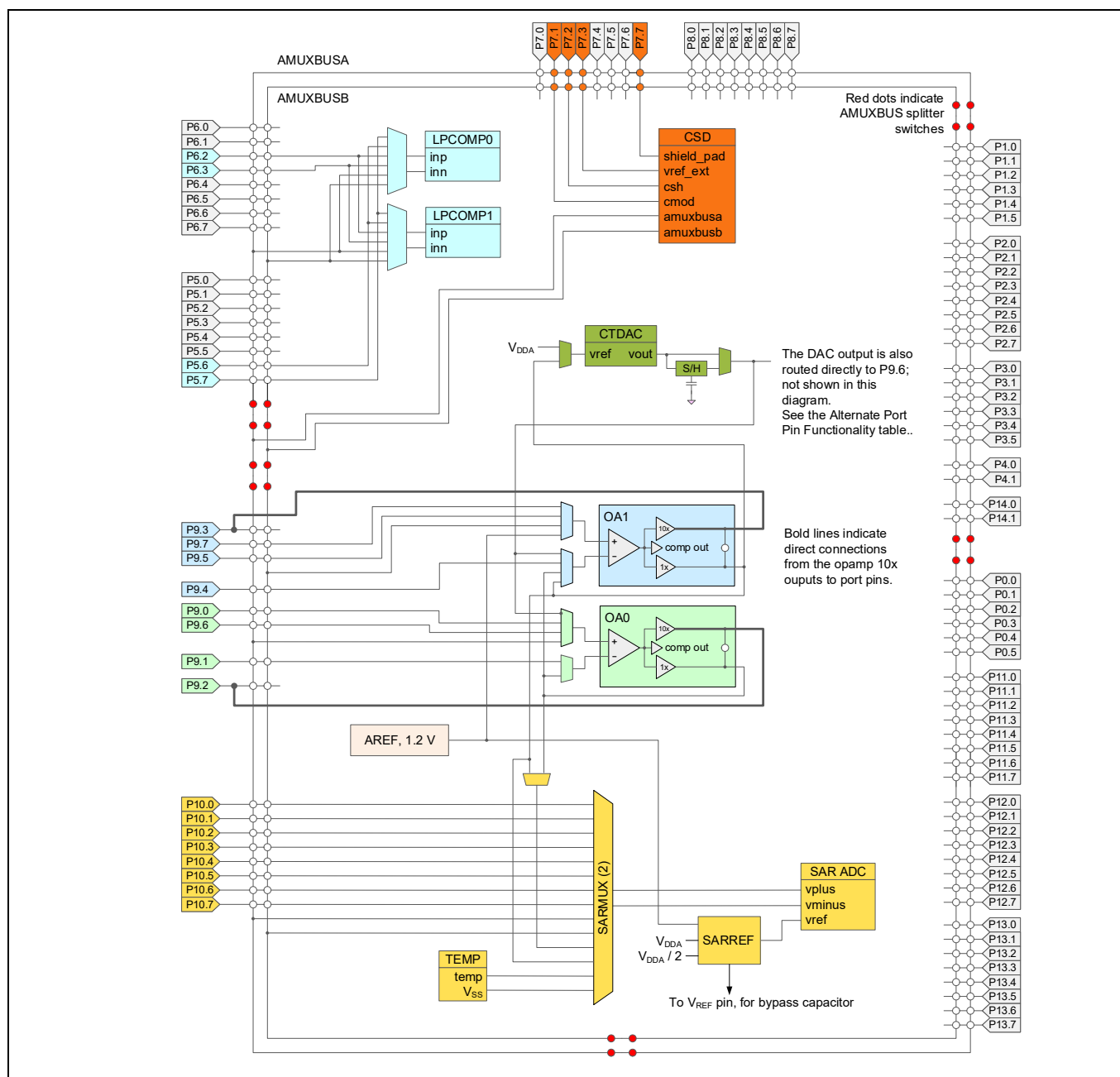
Figure 7 Analog subsystem
