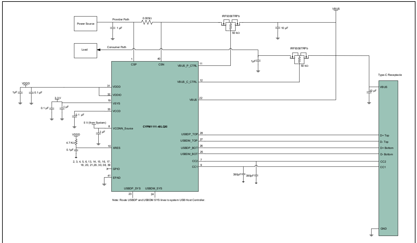
Figure 10 EZ-PD™ PMG1-S1-based DRP application diagram
