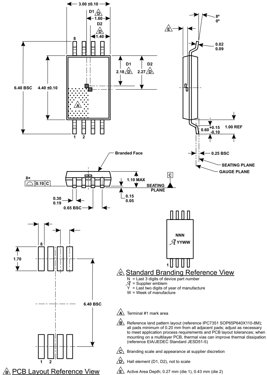
Figure 38: Package LE, 8-Pin TSSOP (Dual Die Version)
