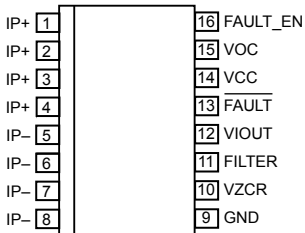
Pinout Diagram
