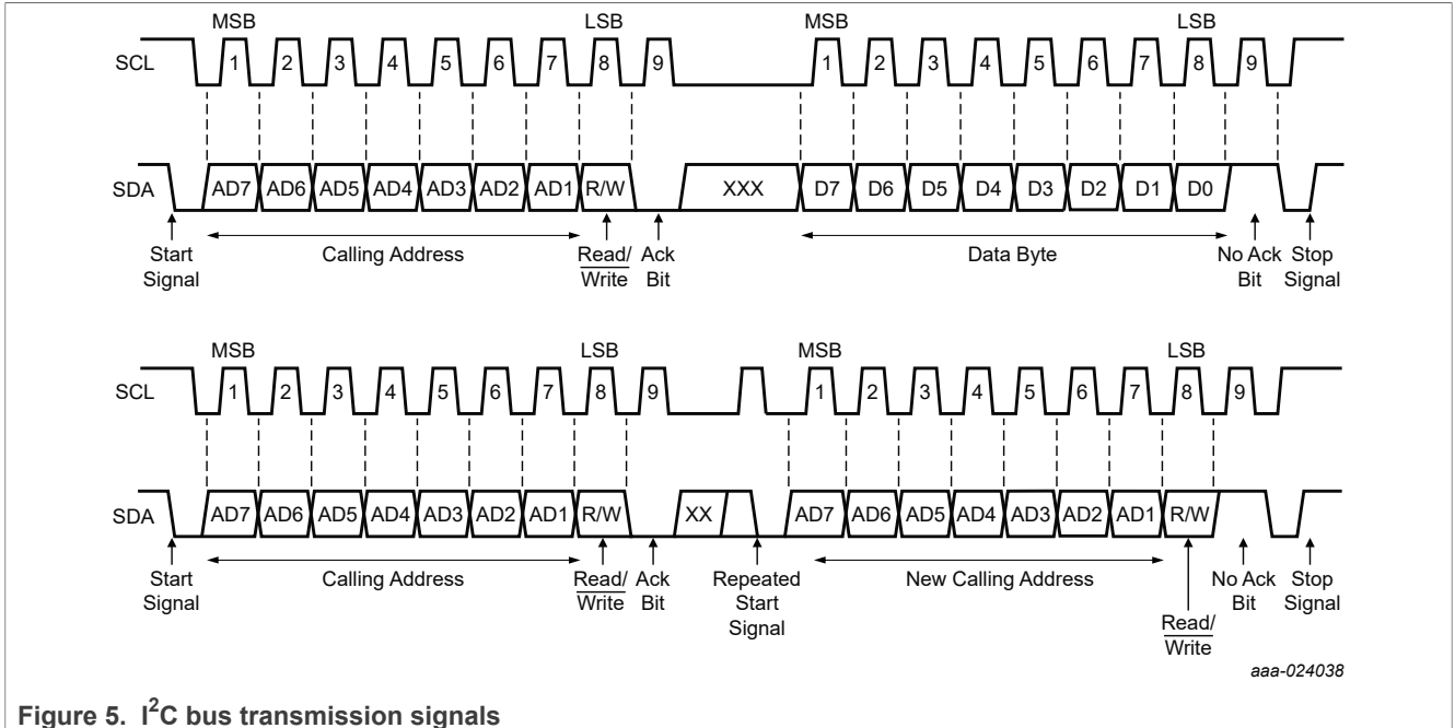
Figure 5. I 2 C bus transmission signals
