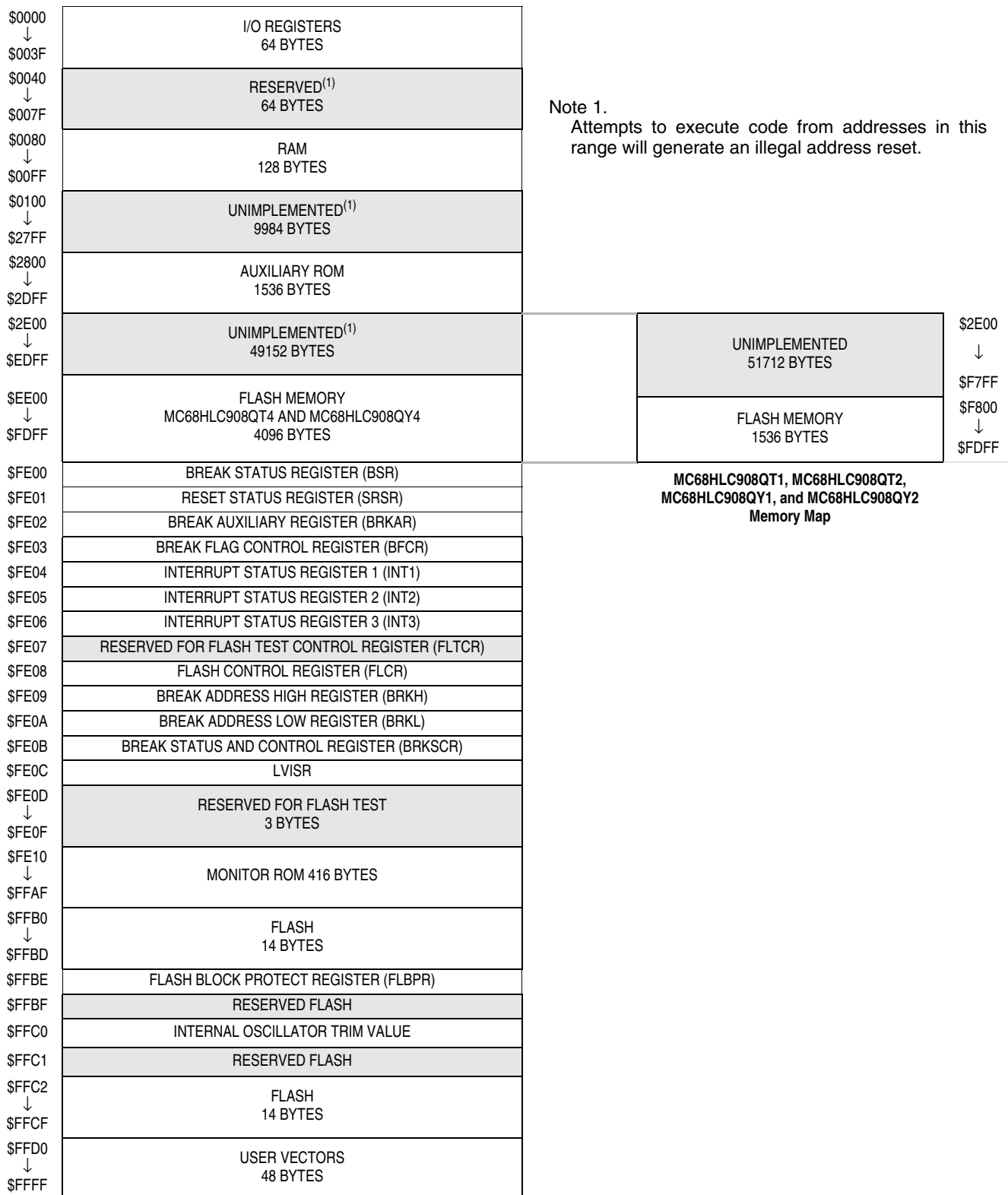
Figure 2-1. Memory Map
