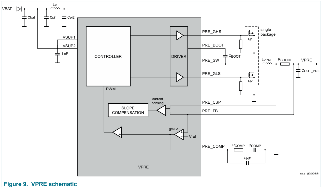
Figure 9. VPRES schematic
