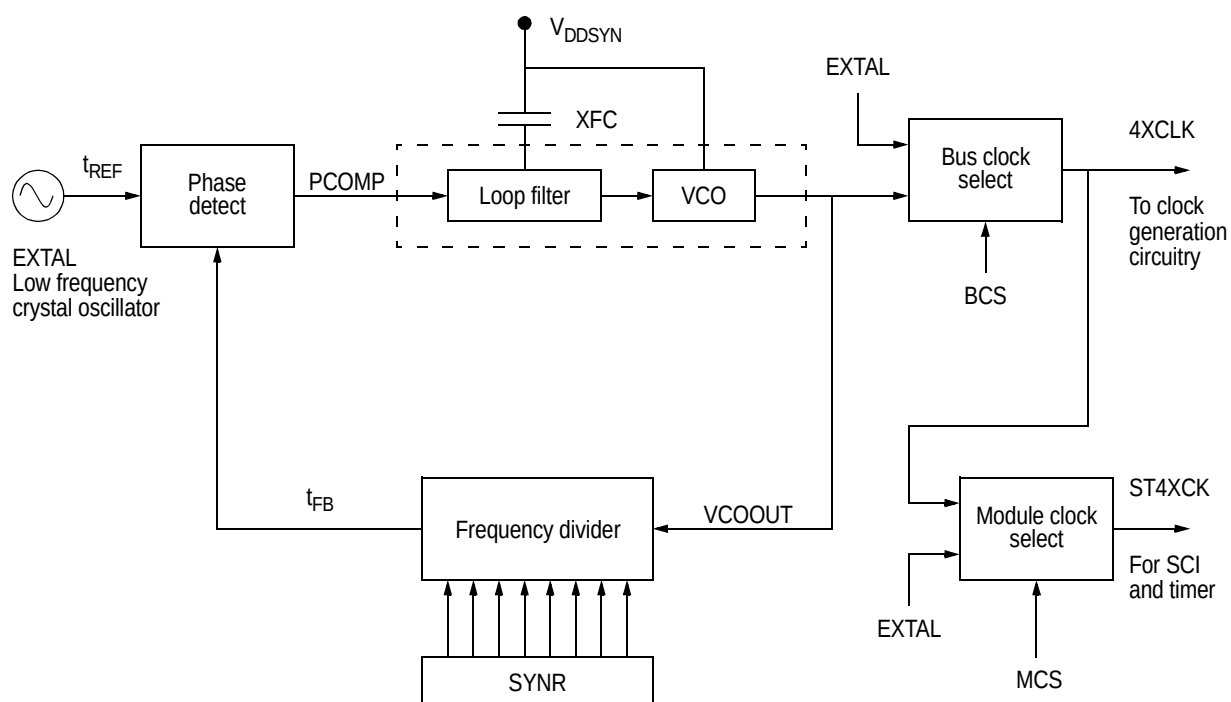
Figure 2-4. PLL circuit
