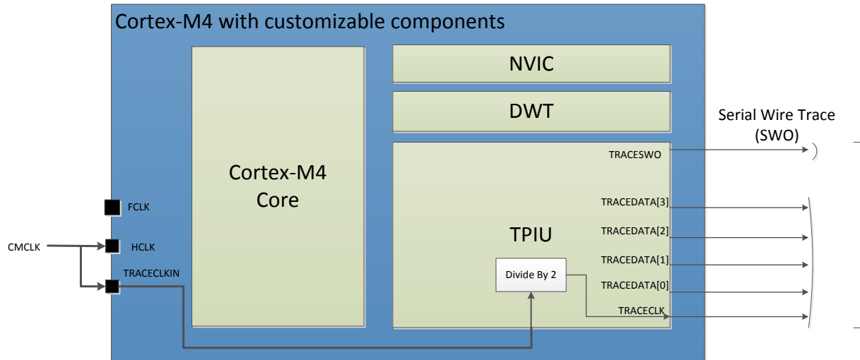
Figure 7-111. Debug Trace
