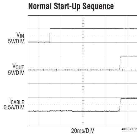
FIGURE 4 CIRCUIT R_{\text{IN}} = 150\text{m}\Omega , L_{\text{IN}} = 0.7\mu\text{H} \text{LOAD} = 10\Omega , C_{\text{OUT}} = 10\mu\text{F}
