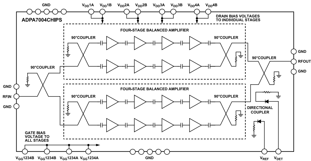
Figure 45. Simplified Block Diagram
