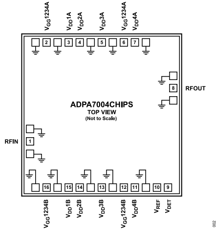
Figure 2. Pad Configuration
