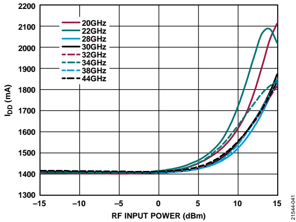
Figure 41. I_{DD} vs. RF Input Power at Various Frequencies, V_{DD} = 5\text{ V} , I_{DQ} = 1400\text{ mA}
