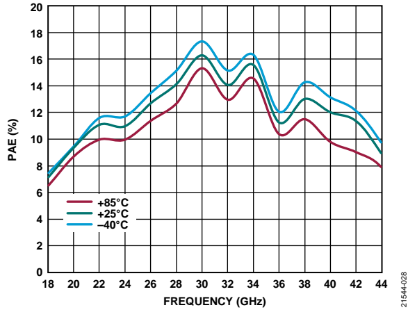
Figure 28. Power Added Efficiency (PAE) vs. Frequency for Various Temperatures, V_{DD} = 5V , I_{DQ} = 1400\text{ mA} , PAE Measured at P_{SAT}
