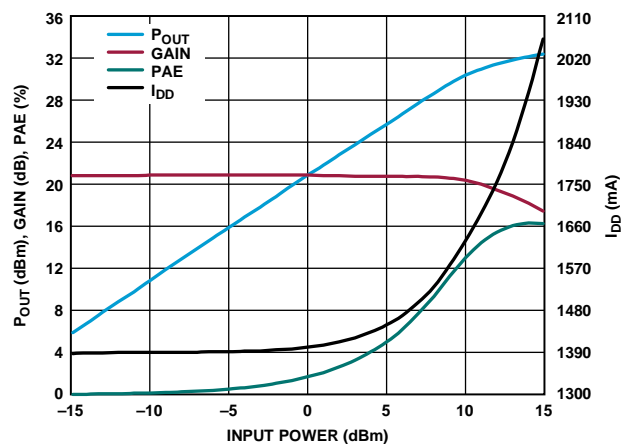
Figure 33. P_{OUT} , Gain, PAE, and I_{DD} vs. Input Power, 30 GHz, V_{DD} = 5V , I_{DD} = 1400\text{ mA}
