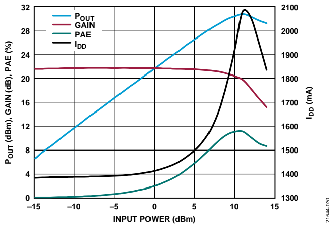
Figure 30. P_{OUT} , Gain, PAE, and Drain Current with RF Applied ( I_{DD} ) vs. Input Power, 22 GHz, V_{DD} = 5V , I_{DD} = 1400\text{ mA}
