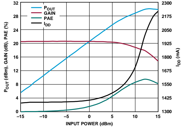
Figure 32. P_{OUT} , Gain, PAE, and I_{DD} vs. Input Power, 20 GHz, V_{DD} = 5V , I_{DD} = 1400\text{ mA}
