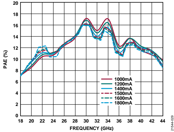
Figure 29. PAE vs. Frequency for Various I_{DQ} , V_{DD} = 5V , I_{DQ} = 1400\text{ mA} , PAE Measured at P_{SAT}
