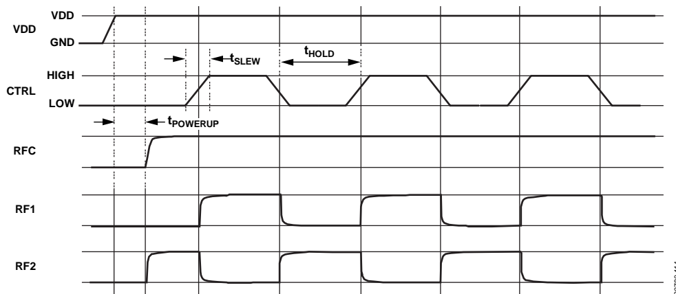
Figure 14. Timing Requirements
