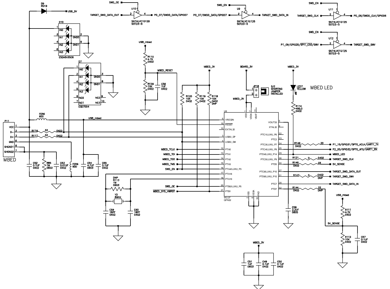
Figure 37. mbed Circuit Schematic
