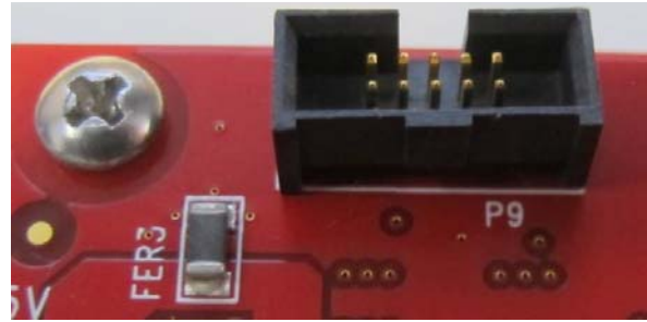
Figure 17. P9 Debug Connector
