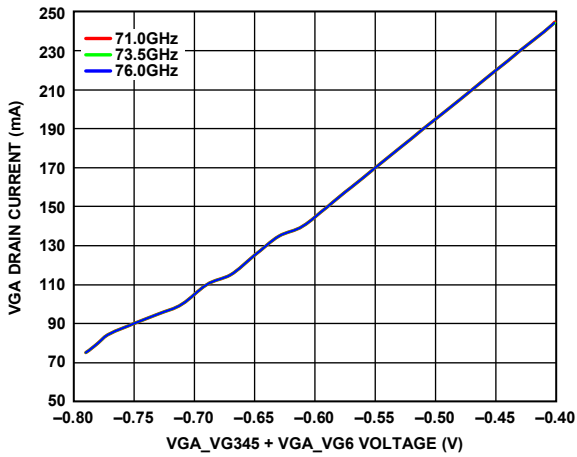
Figure 34. VGA Drain Current vs. VGA\_VG345 + VGA\_VG6 Voltage at Various Frequencies
