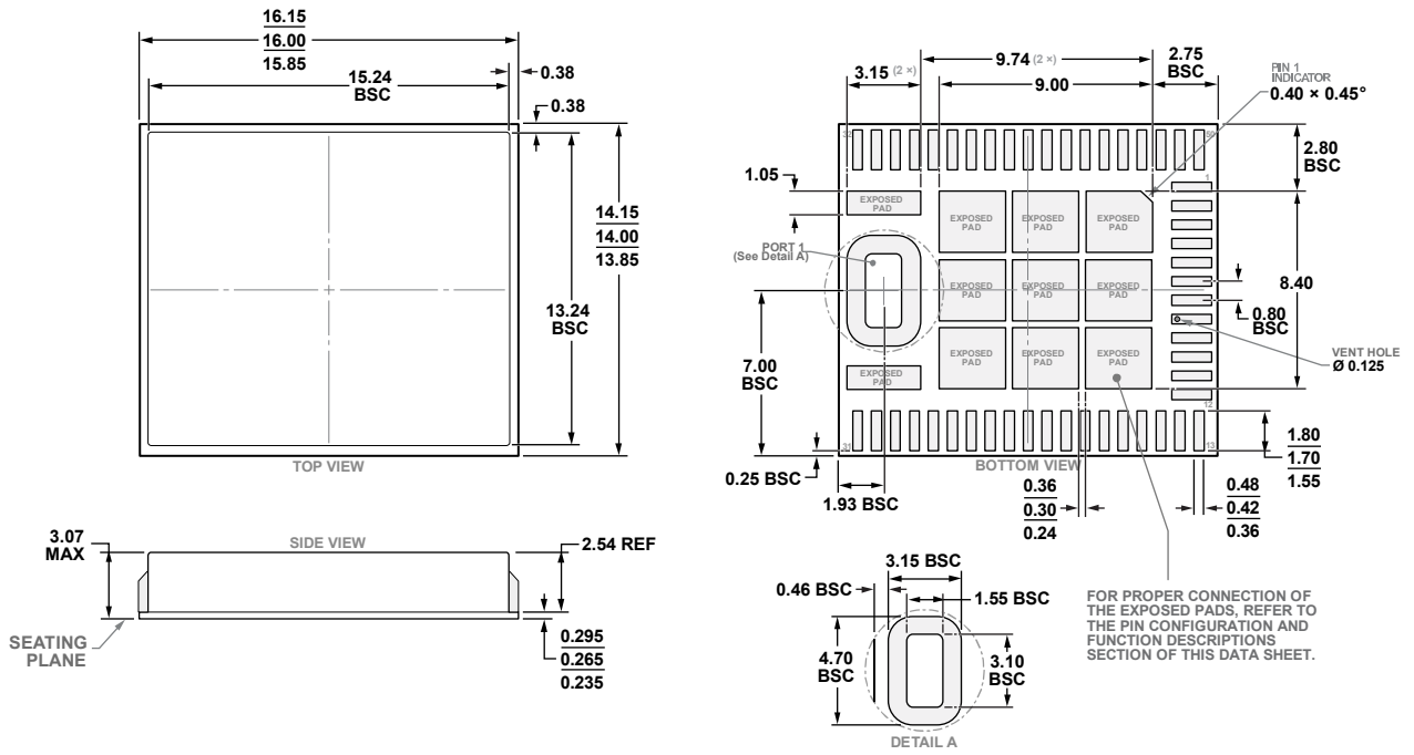
Figure 87. 50-Terminal Chip Array Small Outline No Lead Cavity [LGA_CAV] 16.00 mm x 14.00 mm Body and 3.07 mm Package Height (CE-50-2) Dimensions shown in millimeters
