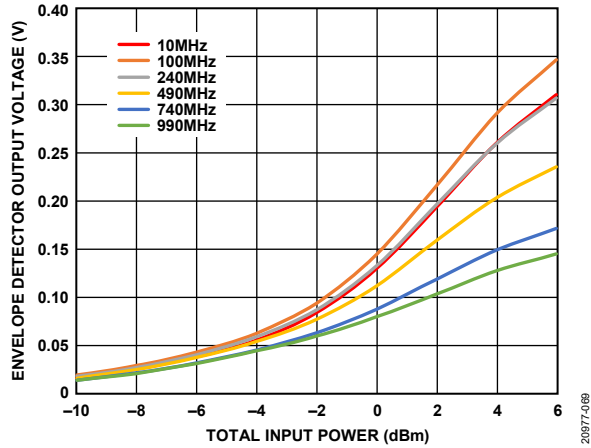
Figure 69. Envelope Detector Output Voltage vs. Total Input Power at Various Input Tone Spacings, RF = 71 GHz
