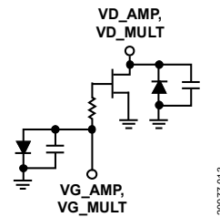
Figure 13. VD_AMP, VD_MULT, VG_AMP, and VG_MULT Interface Schematic
