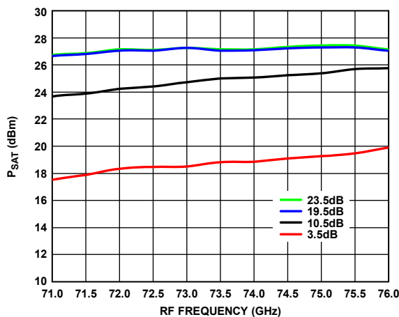
Figure 29. Psat vs. RF Frequency at Various Gains
