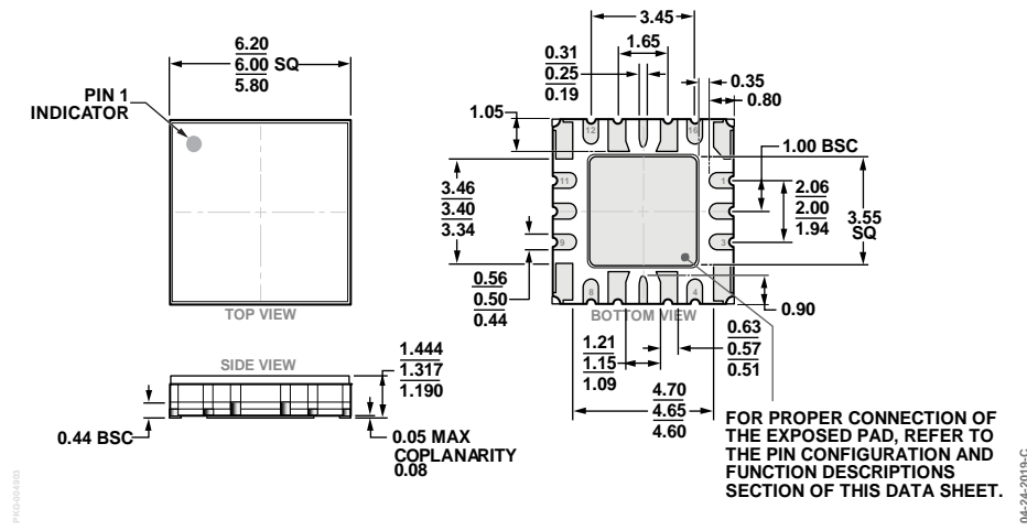
Figure 63. 16-Terminal Ceramic Leadless Chip Carrier with Heat Sink [LCC_HS] (EH-16-1) Dimensions shown in millimeters
