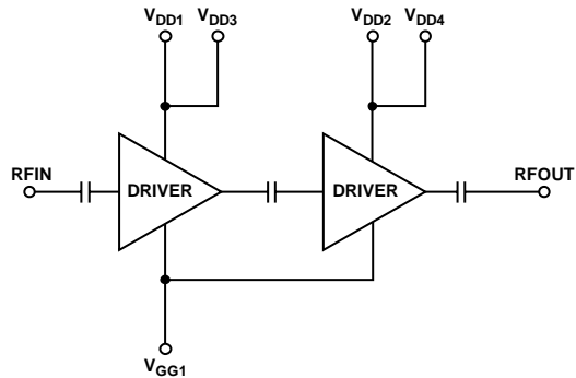
Figure 50. Simplified Architecture
