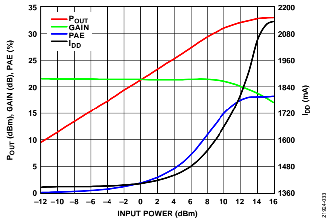
Figure 33. P_{OUT} , Gain, PAE, and I_{DD} vs. Input Power, 30 GHz, V_{DD} = 5V , I_{DD} = 1400mA
