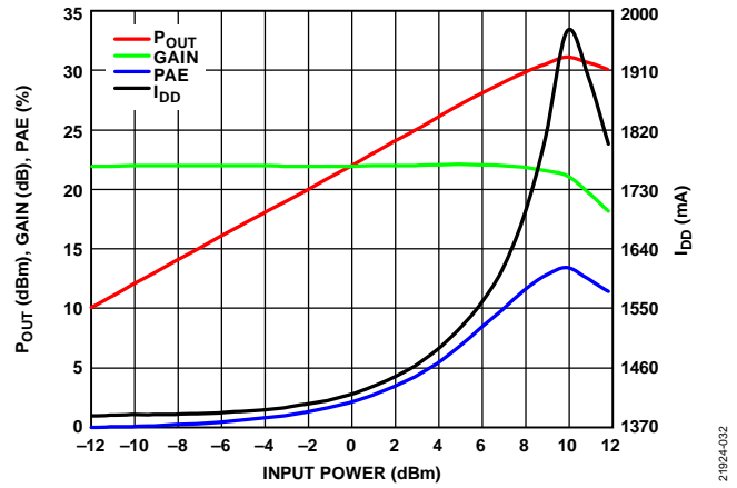
Figure 32. P_{OUT} , Gain, PAE, and I_{DD} vs. Input Power, 22 GHz, V_{DD} = 5V , I_{DD} = 1400mA
