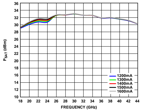
Figure 27. P_{SAT} vs. Frequency for Various Supply Currents, V_{DD} = 5V
