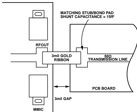
Figure 54. High Frequency Output Wideband Matching
