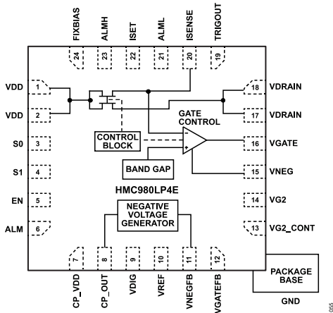
Figure 54. HMC980LP4E Active Bias Control
