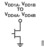
Figure 9. V DD1A , V DD1B to V DD4A , V DD4B Interface Schematic
