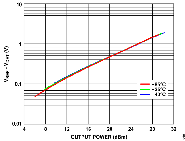
Figure 46. Detector Voltage ( V_{REF} - V_{DET} ) vs. Output Power for Various Temperatures at 32 GHz, V_{DD} = 5 V, I_{DQ} = 800 mA
