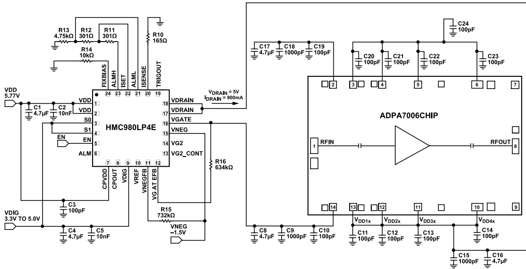
Figure 56. Application Circuit Using the HMC980LP4E with the ADPA7006CHIP (External Negative Voltage Source)
