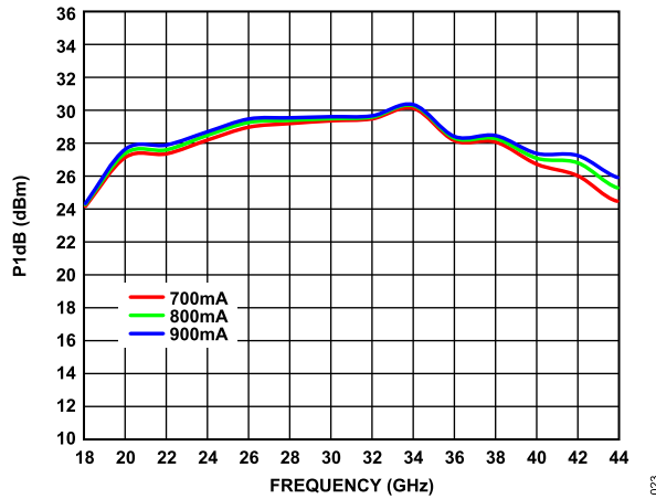
Figure 23. P_{1dB} vs. Frequency for Various Supply Currents ( I_{DQ} ), V_{DD} = 5\text{ V}
