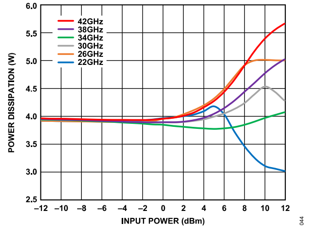
Figure 44. Power Dissipation vs. Input Power at T = 85^{\circ}\text{C} , V_{DD} = 5 V, I_{DQ} = 800 mA
