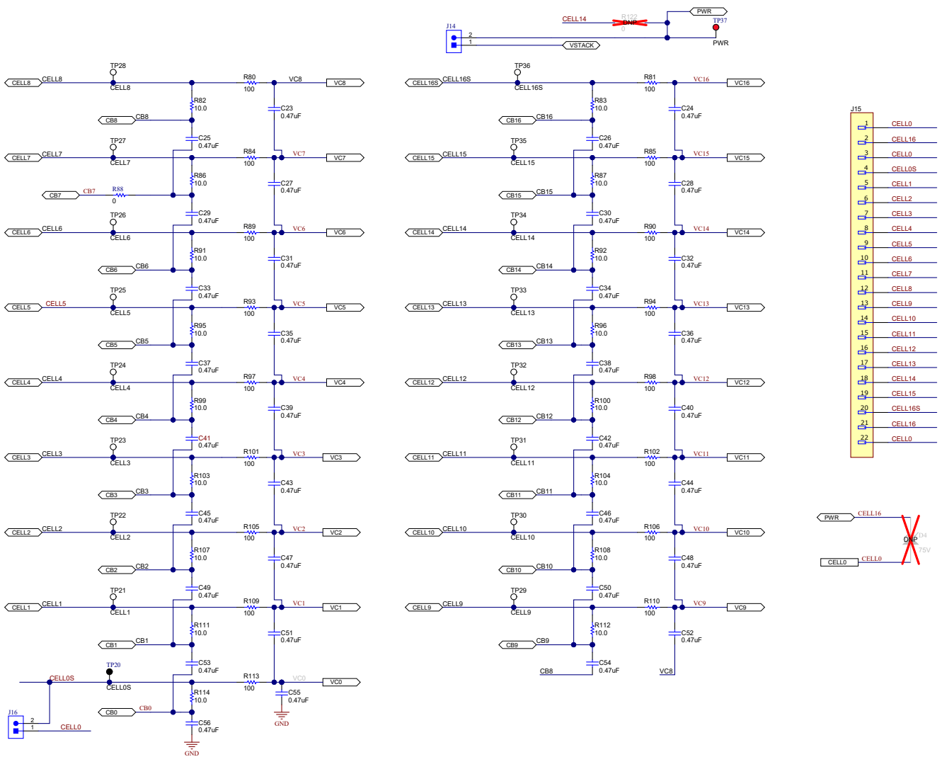
Figure 9-3. BQ79656EVM Schematic Part 2
